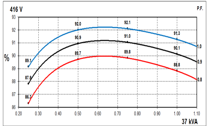
60Hz Curves
