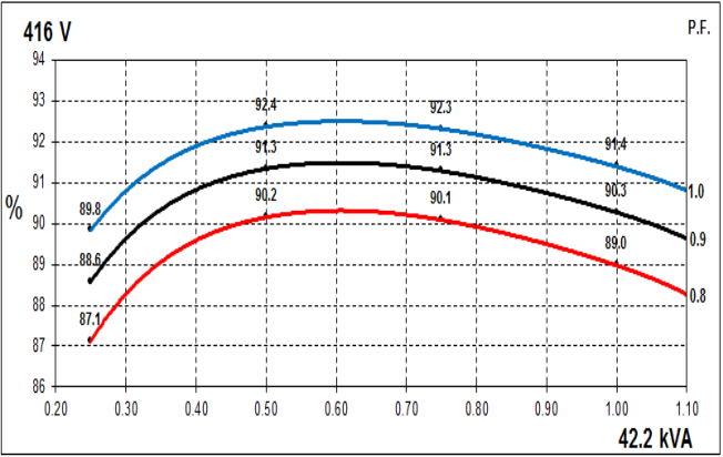
60Hz Curves
