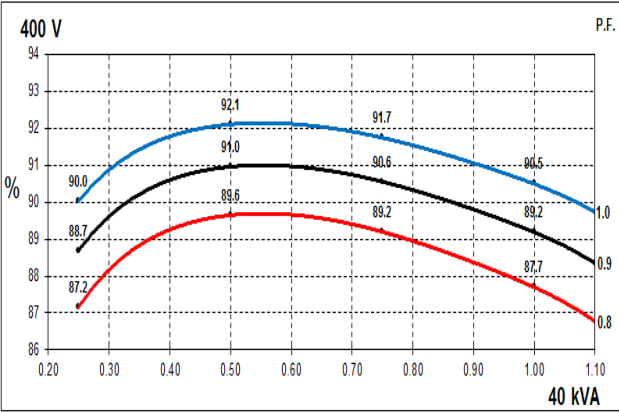
50Hz Curves
