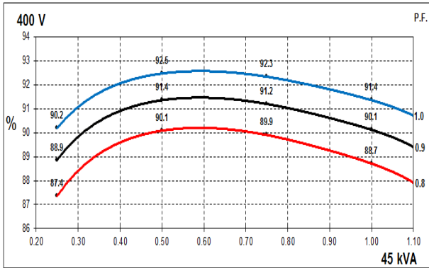
50Hz Curves
