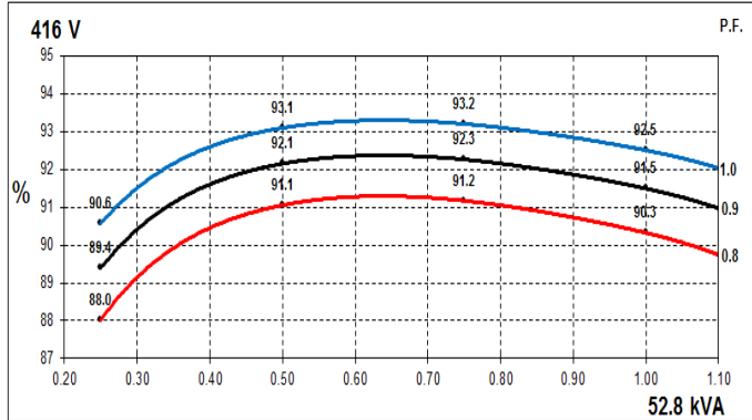
60Hz Curves
